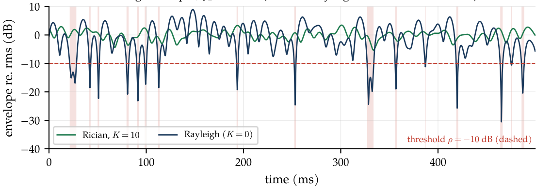
Fading envelopes, f_D = 50 Hz (shaded: Rayleigh fades below threshold)
