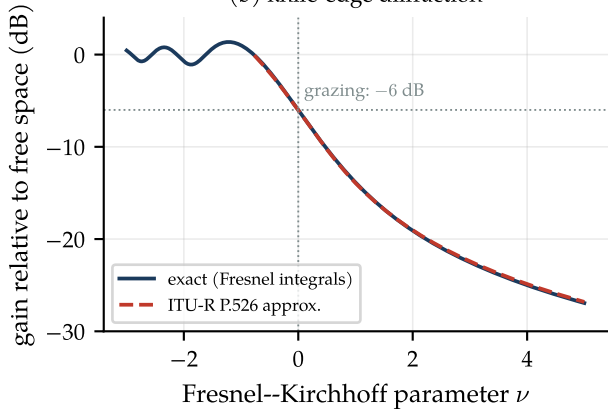
(b) knife-edge diffraction
