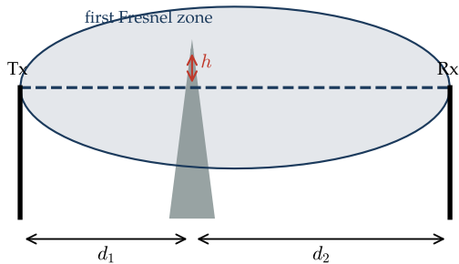
(a) knife-edge geometry
