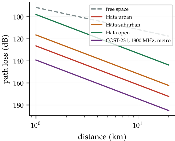
(a) 900 MHz, h_b = 30 m, h_m = 1.5 m
