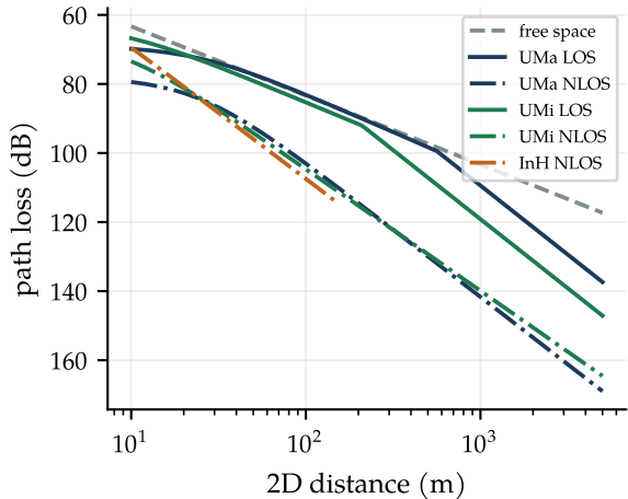
(b) 3GPP TR 38.901, 3.5 GHz
