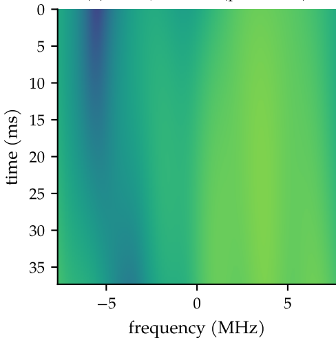
(a) EPA, f_D = 5 Hz (pedestrian)
