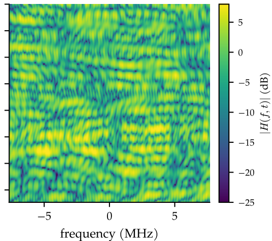
(b) ETU, f_D = 300 Hz (vehicular)
