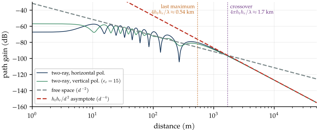
Two-ray ground reflection, 900 MHz, h_t = 30 m, h_r = 1.5 m
