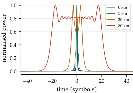
one 64-GBd pulse after SMF ( D = 17 ps/nm/km)
