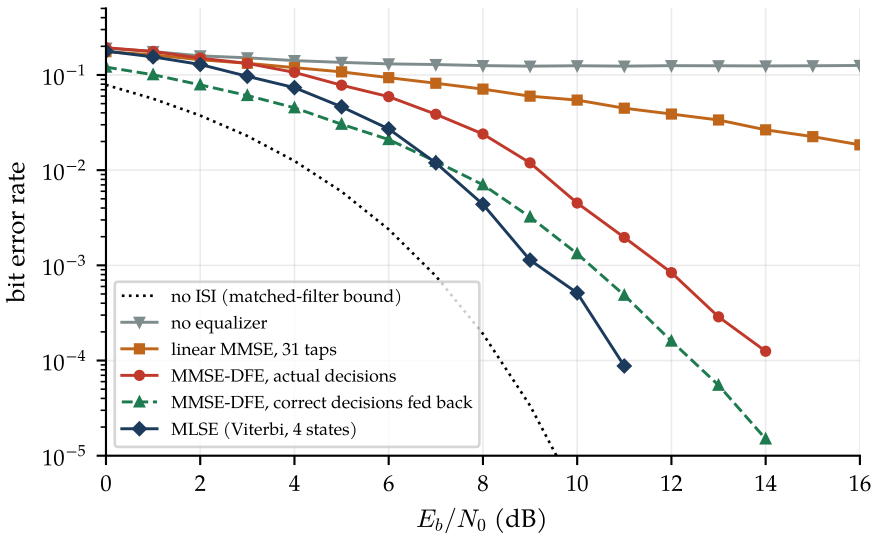
BPSK over Proakis channel B [0.407, 0.815, 0.407]
