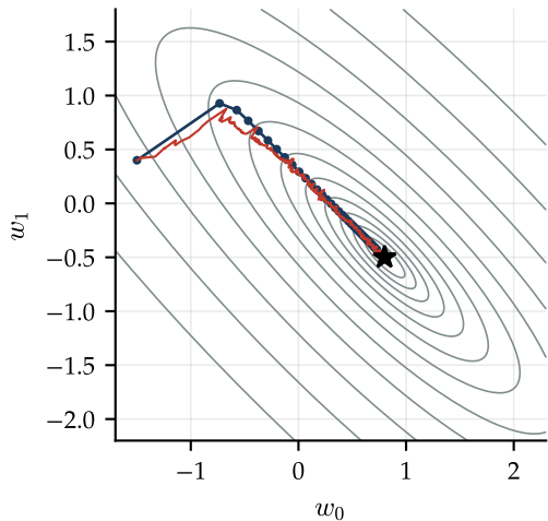
\rho = 0.85 : eigenvalue spread \chi = 12.3
