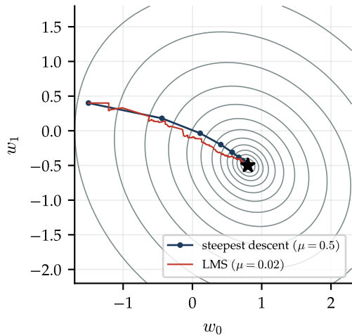
\rho = 0.2 : eigenvalue spread \chi = 1.5
