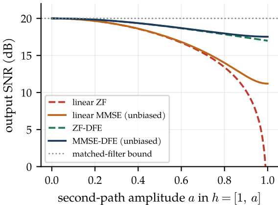
two-path channel, SNR = 20 dB
