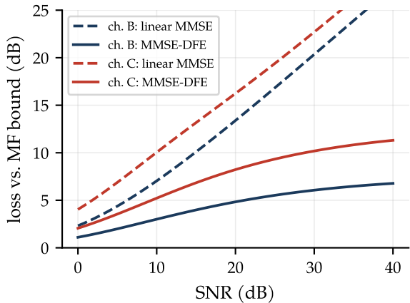
Proakis channels B and C
