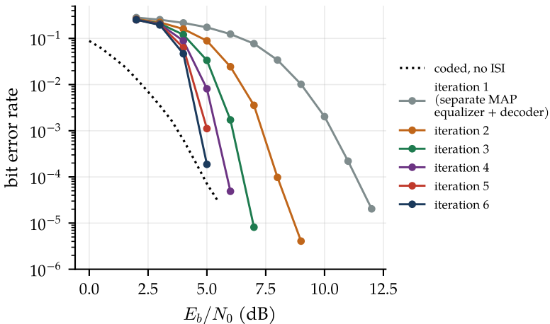
turbo equalization: (7,5) code, Proakis C, 1024-bit frames
