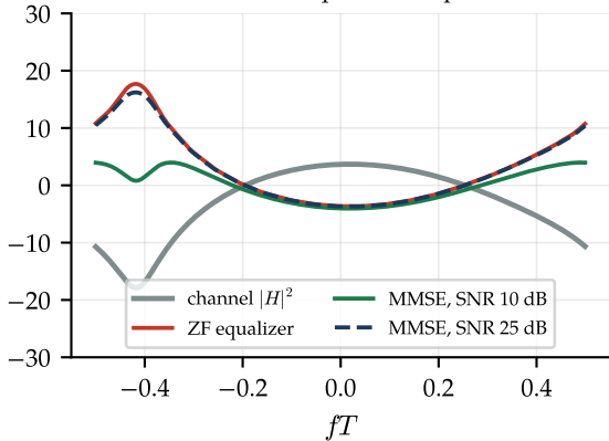
channel and equalizer responses
