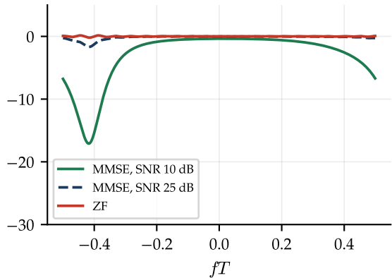
overall response |HW|^2
