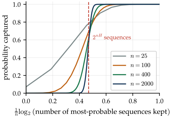
(b) 2^{nH} of 2^n sequences suffice
