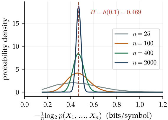
(a) Sample entropy concentrates
