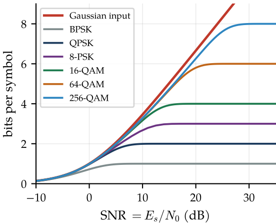
(a) Constrained-input capacity
