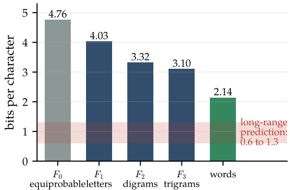
(b) Entropy of English (27 symbols)
