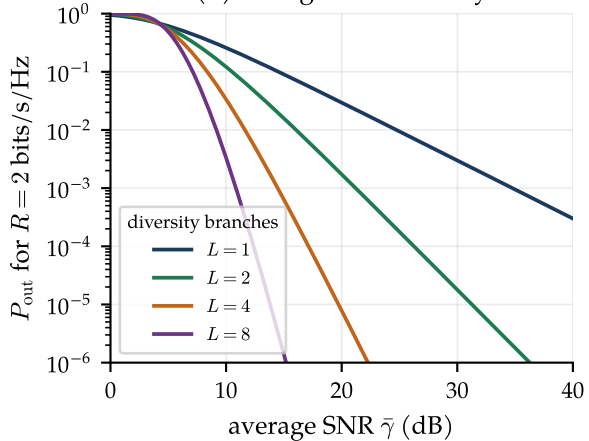
(b) Outage and diversity
