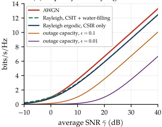
(a) Capacity of a Rayleigh channel
