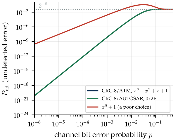
8-bit CRCs, 64-bit message
