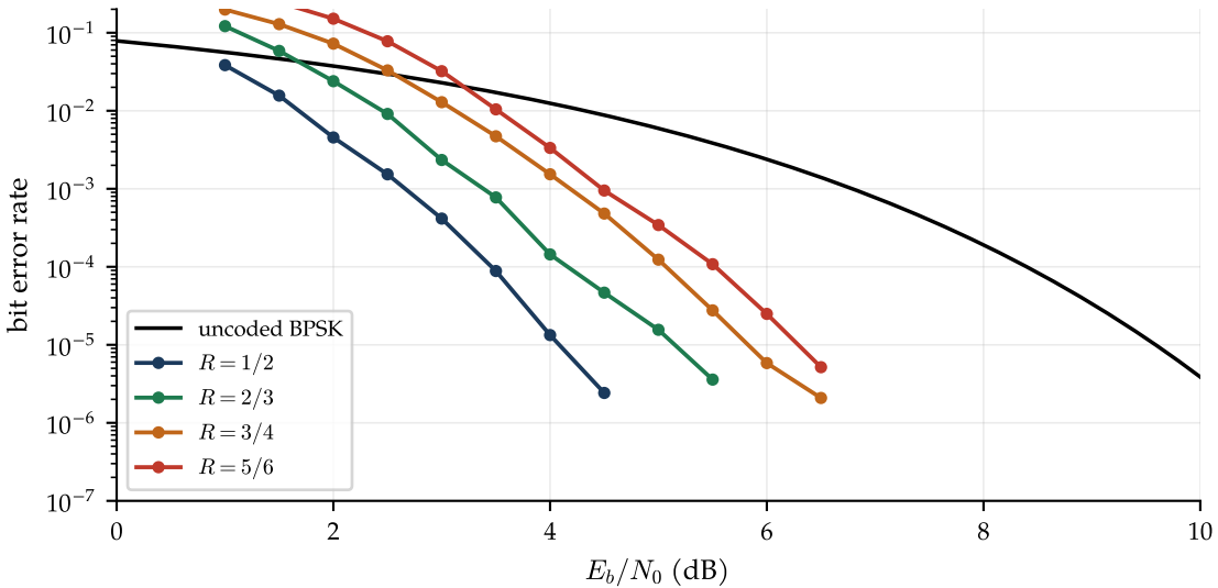
The K = 7 code punctured as in IEEE 802.11 (soft Viterbi)
