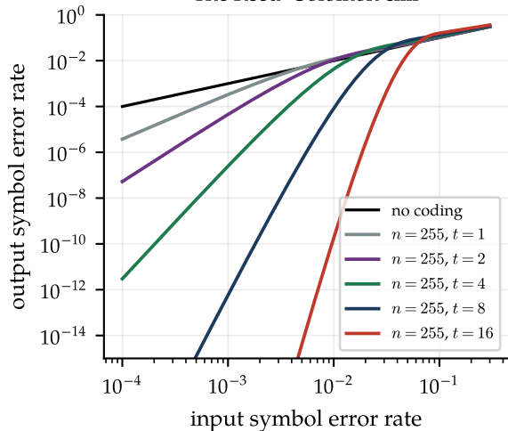
The Reed-Solomon cliff
