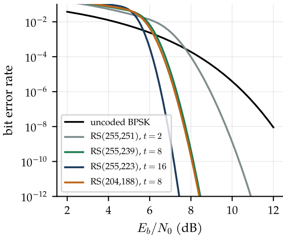
RS codes over GF(256), BPSK, hard
