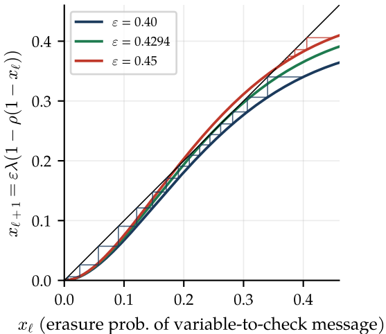
(a) (3,6) ensemble on the BEC
