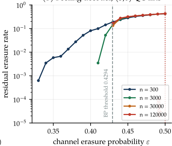
(b) Peeling decoder, (3,6) QC lifts
