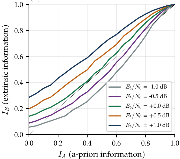
(a) Transfer curves of one RSC decoder
