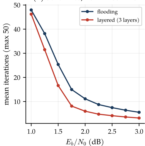
(b) Schedules, normalised MS
