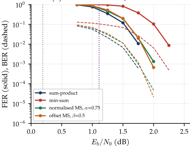
(a) Check-node rules, 50 iterations
