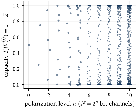
(a) Splitting BEC(0.5), level by level
