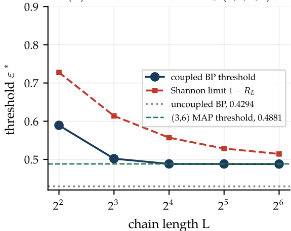
(b) Threshold saturation, (3,6,L,3)
