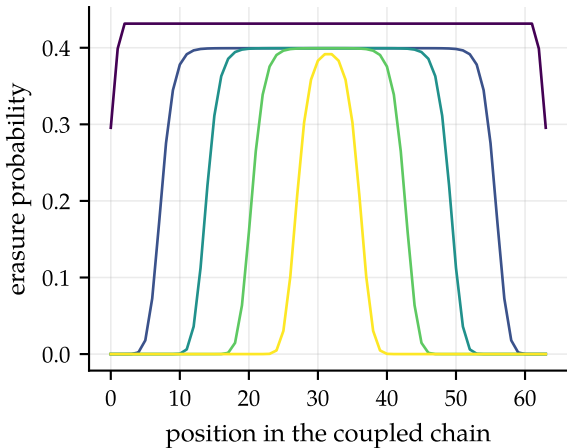
(a) Decoding wave, \varepsilon = 0.47 , L = 64
