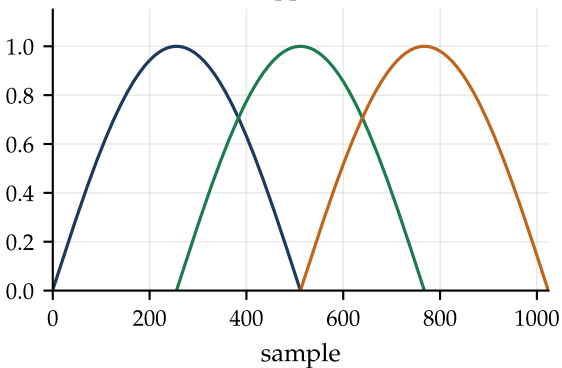
(a) 50%-overlapped sine windows
