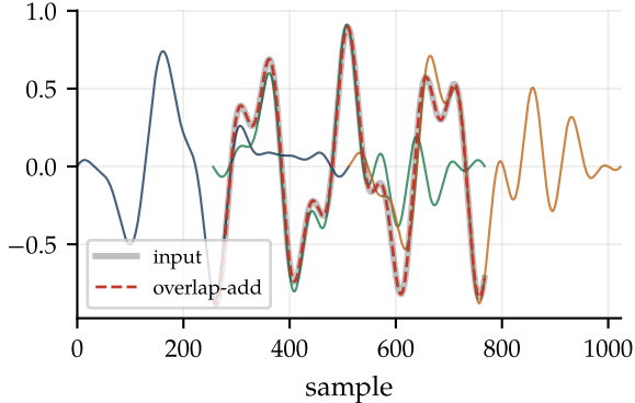
(b) Each block aliases; the sum is exact
