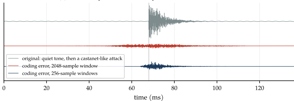
(c) Pre-echo: quantisation noise spreads over the whole window
