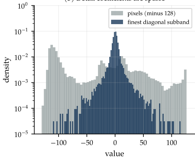
(b) Detail coefficients are sparse
