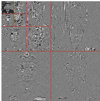
(a) Three-level 5/3 wavelet transform
