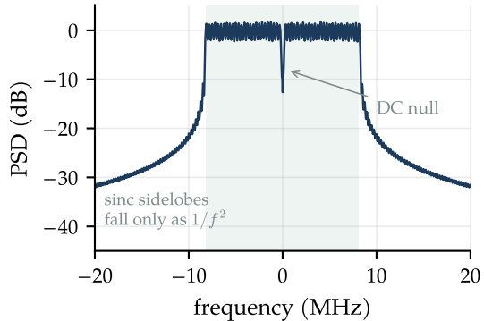
(b) Spectrum: 52 subcarriers, 16.6 MHz
