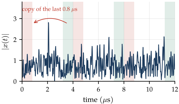
(a) Three 4\ \mu\text{s} symbols: CP (shaded) + 3.2\ \mu\text{s}
