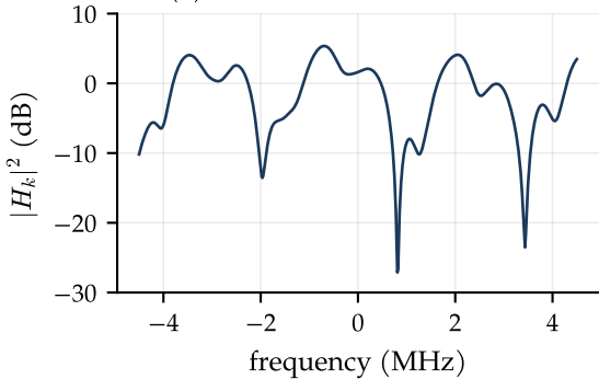
(a) EVA channel, 600 subcarriers
