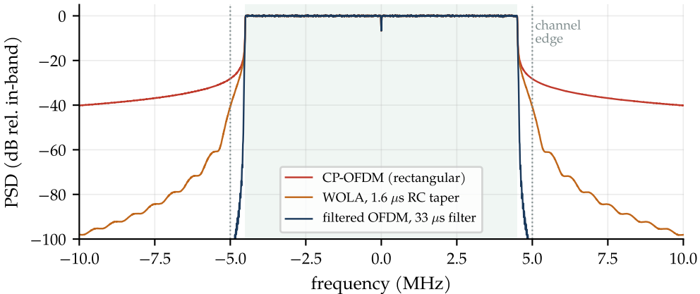
600 subcarriers of 15 kHz (9 MHz) in a 10 MHz channel
