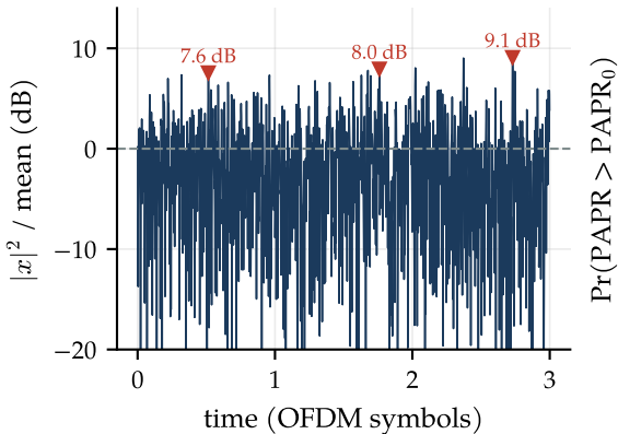
(a) Instantaneous power, 200 QPSK subcarriers
