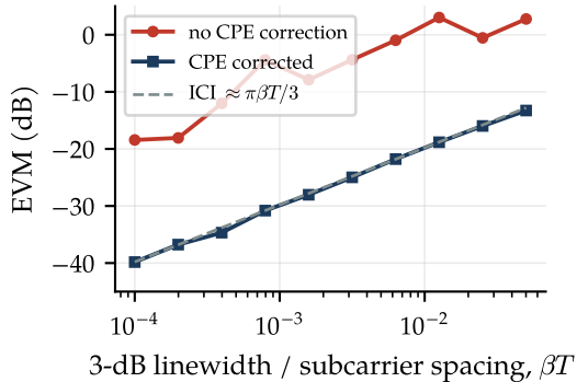
(c) Error vector magnitude
