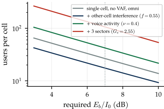
(a) IS-95 uplink pole capacity
