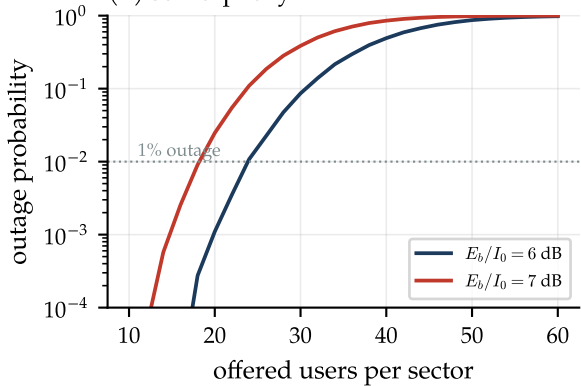
(b) soft capacity
