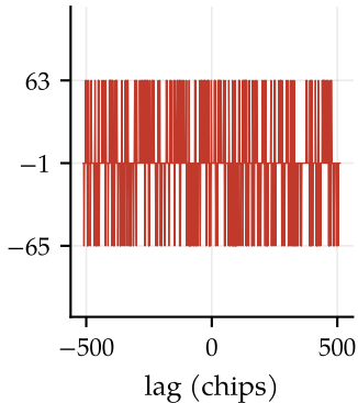
(b) PRN 1 \times PRN 2
