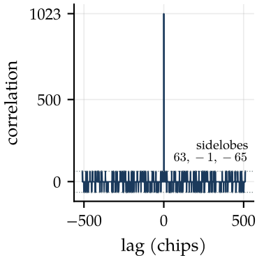
(a) PRN 1 autocorrelation
