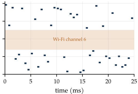
(b) adaptive hopping avoids Wi-Fi
