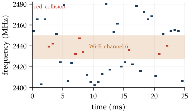
(a) hopping over all 79 channels
