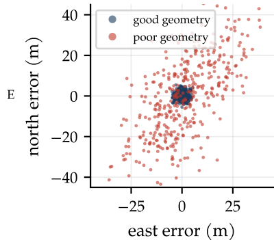
(c) fixes, \sigma_{\text{UERE}} = 3 \text{ m}
