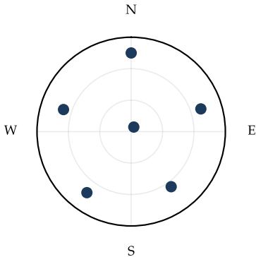
(a) good geometry PDOP 1.9, HDOP 1.0
