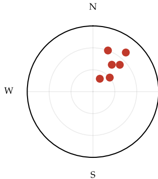
(b) poor geometry PDOP 12.0, HDOP 8.8
