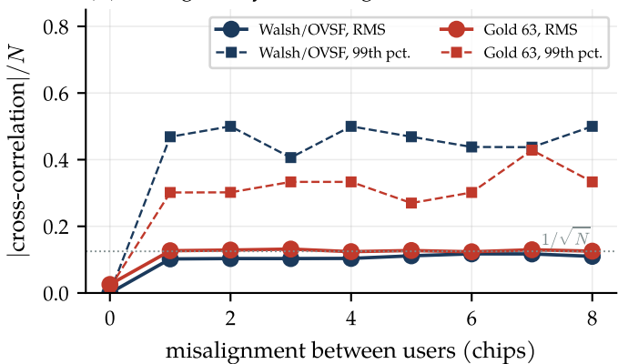
(b) orthogonality needs alignment
