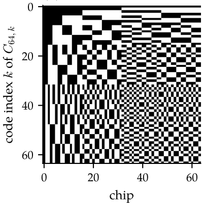
(a) OVSF codes, SF 64
