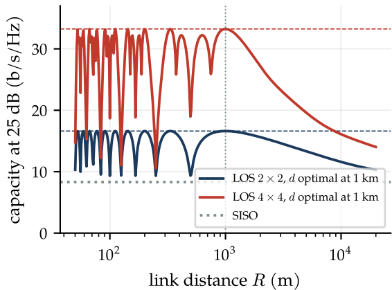
(b) capacity vs range
