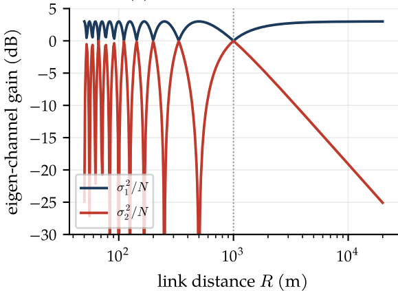
(a) 2 \times 2 , 80 GHz, d = 1.37 m
