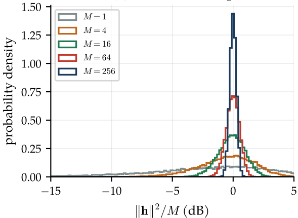
(a) channel hardening
