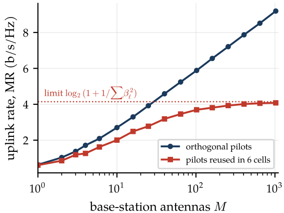
(b) pilot contamination
