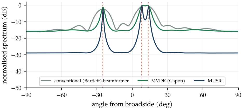
10-element \lambda/2 array, sources at -25^\circ , 8^\circ , 14^\circ ; SNR 5 dB, 200 snapshots
