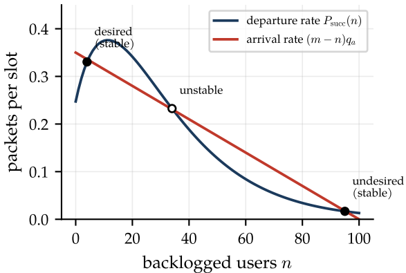
(a) drift, m = 100 , q_r = 0.06
