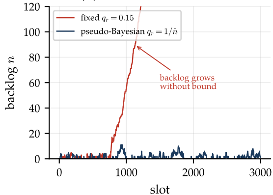
(b) Poisson arrivals, \lambda = 0.3
