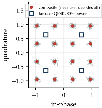
(b) superposed constellation
