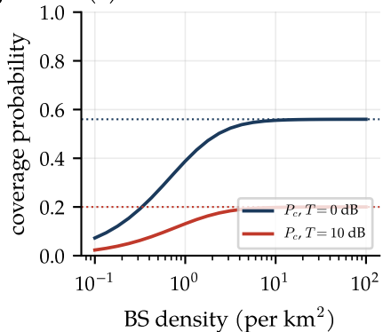
(c) densification with noise
