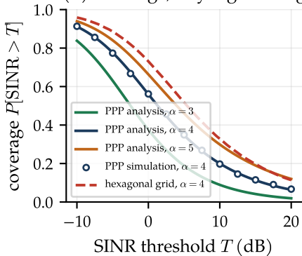
(b) coverage, Rayleigh fading
