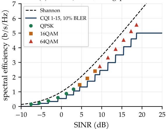
(a) LTE CQI table, 2 dB gap model
