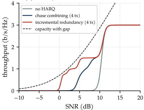
(b) HARQ, first transmission at 3 b/s/Hz
