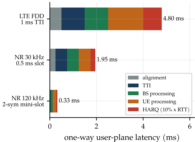
(b) Downlink air-interface budget
