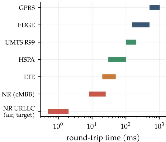
(a) Typical RTT, approximate
