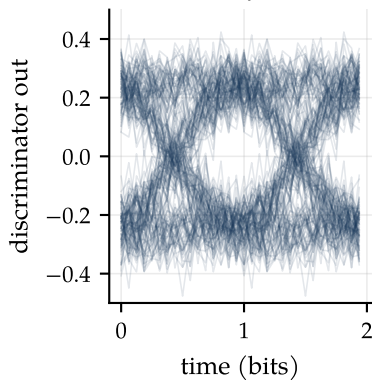
Discriminator eye, SNR 20 dB
