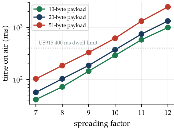
Time on air, 125 kHz, CR 4/5
