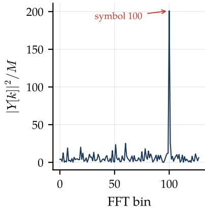
Dechirp + FFT at SNR -7.5 dB
