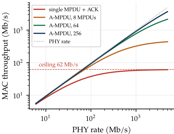
Throughput, 1500-byte packets
