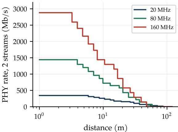
Rate versus range (indoor, n = 3.5 )
