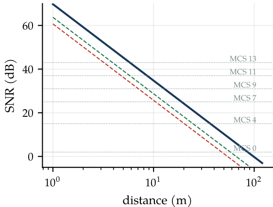
SNR (solid 20 MHz; dashed 80, 160 MHz)
