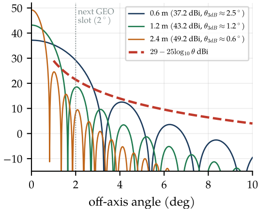
reflector patterns at 14.25 GHz
