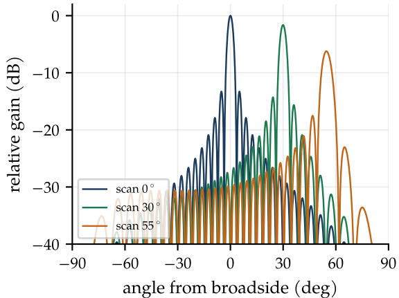
32-element array, \cos^{1.3} element
