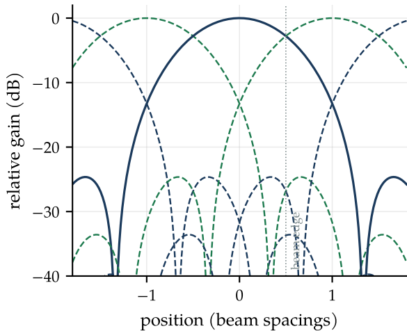
co-channel beams are two spacings apart
